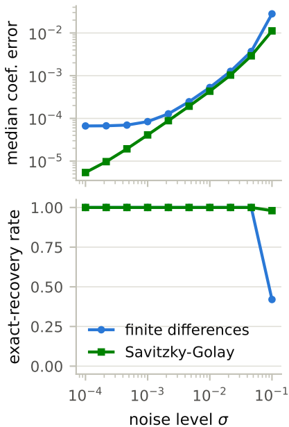
damped oscillator
