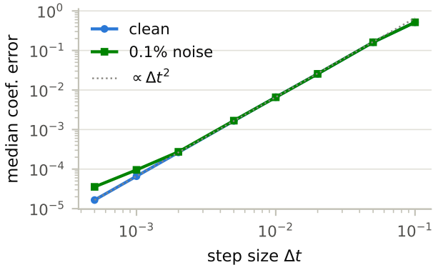
Lorenz, finite differences
