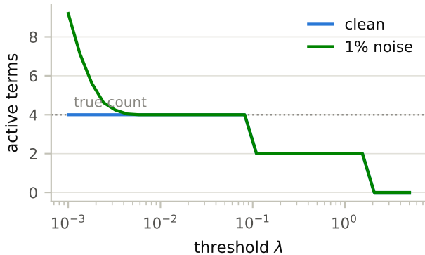
damped oscillator
