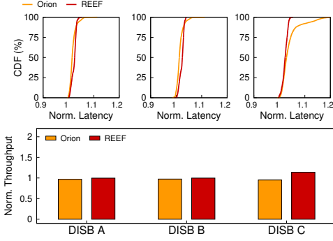
Fig. 29. Comparison of (a) normalized end-to-end latency for RT tasks, and (b) normalized overall throughput of all tasks using Orion [95] and REEF. Both Orion and REEF use the PyTorch [77] to execute DNN models. Testbed: One NVIDIA GV100 GPU.
