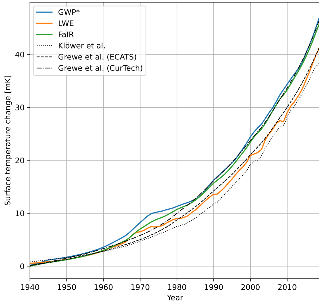
(a) Aviation total climate impacts
