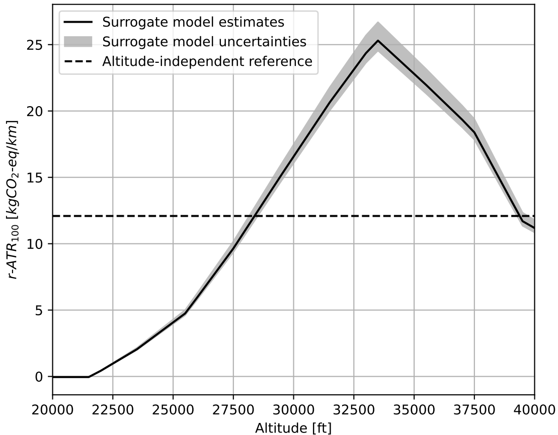
Contrails
