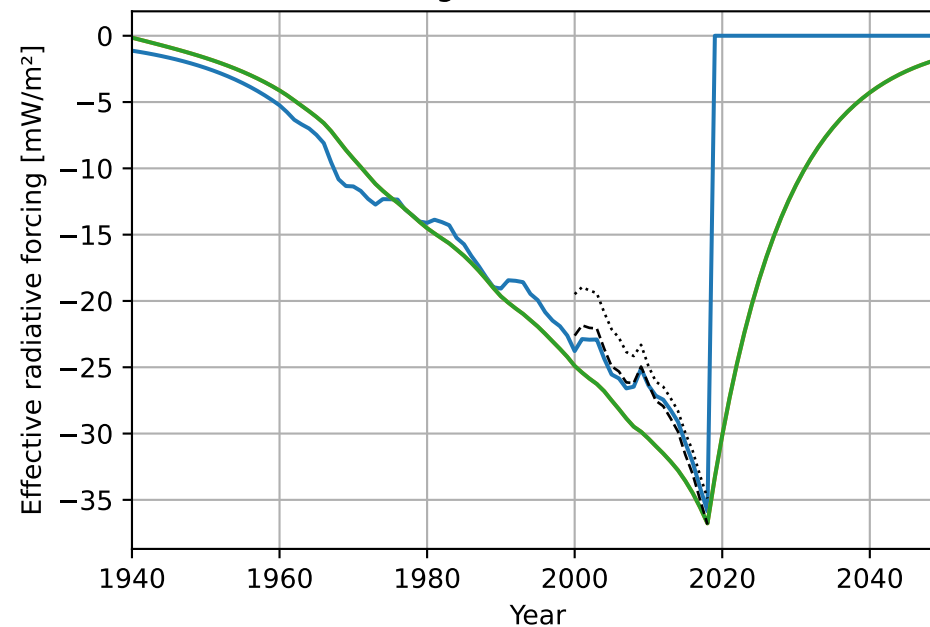
(b) NOx - Long-term methane decrease
