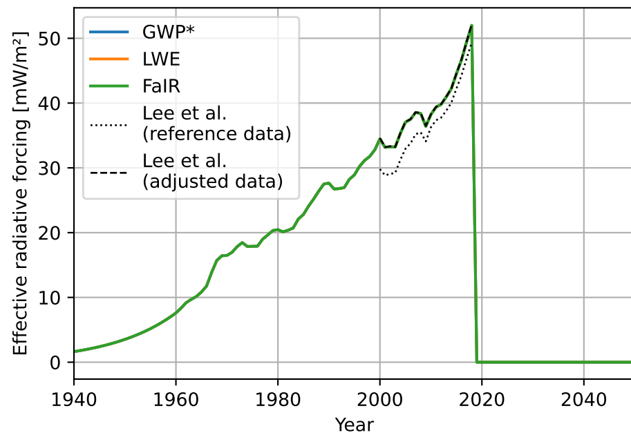
(a) NOx - Short-term ozone increase
