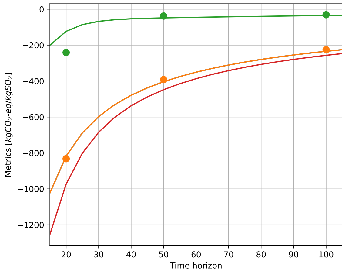
(f) Sulfur
