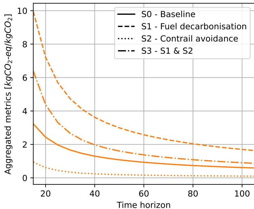
(a) GWP_{ERF}
