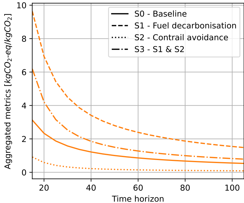
(a) GWP_{ERF}
