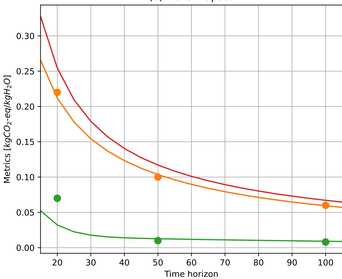
(f) Sulfur
