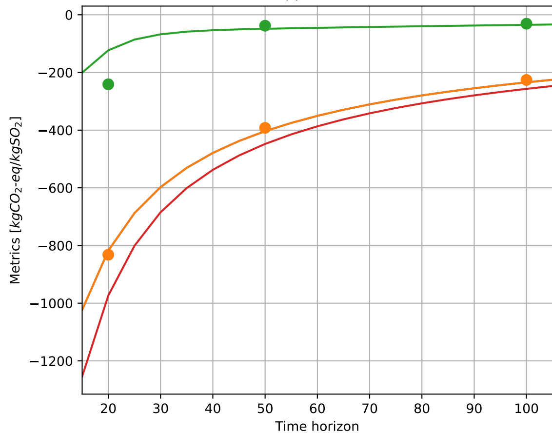
(f) Sulfur
