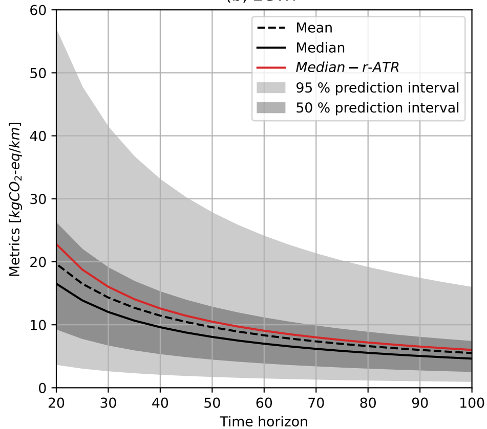
(b) EGWP
