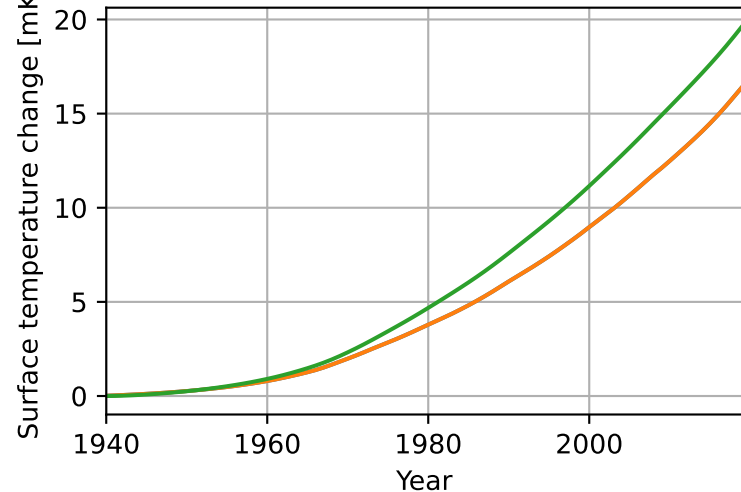
(c) Aviation non-CO 2 climate impacts
