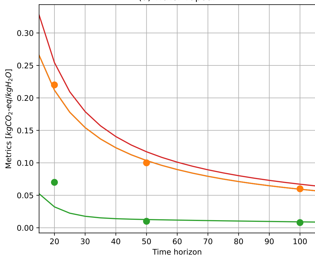
(f) Sulfur
