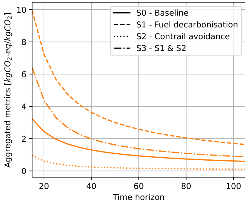
(a) GWP_{ERF}
