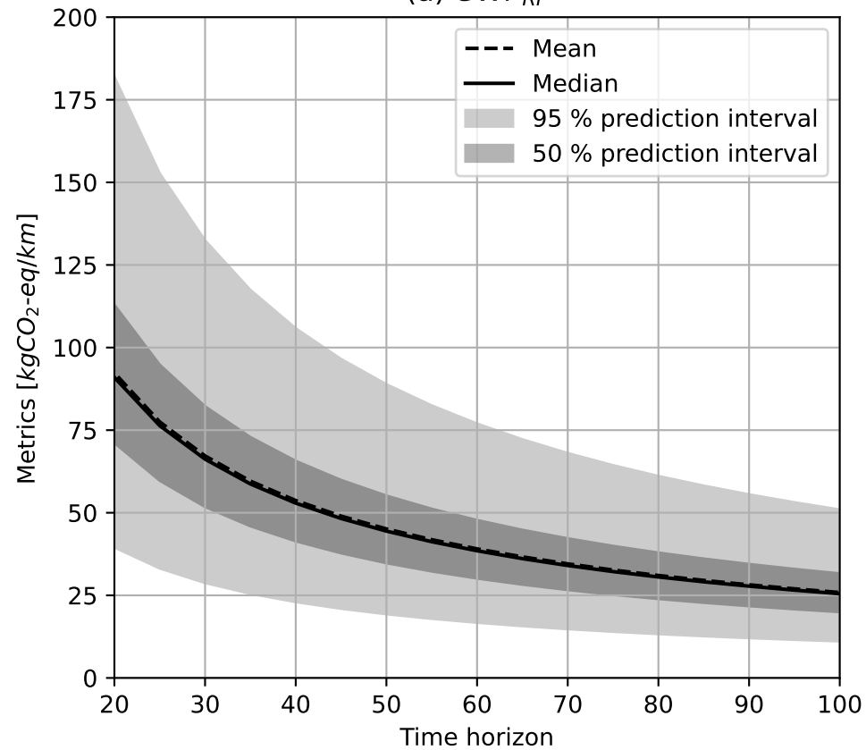
(a) GWP_{RF}
