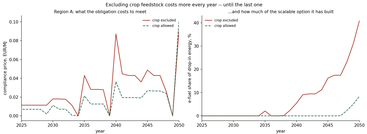
Figure 7: The cost, and the reason for it. Left: the exclusion is dearer in every year until the last; the sawtooth is each obligation step landing and the market catching up. Right: what it bought — a built-out e-fuel industry.
