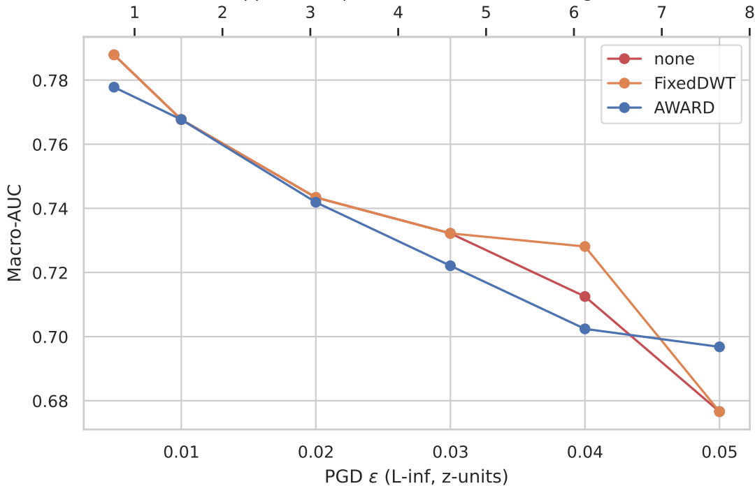
Adaptive robustness vs epsilon (stratified test subset)
