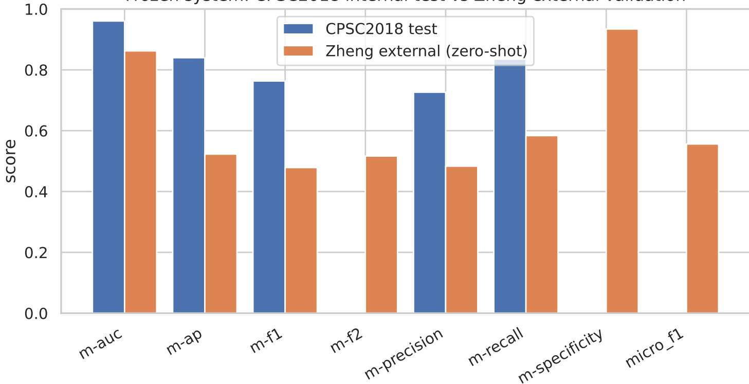
Frozen system: CPSC2018 internal test vs Zheng external validation
