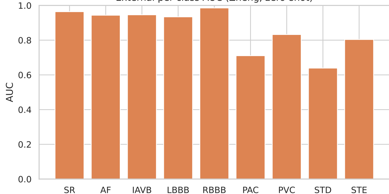
External per-class AUC (Zheng, zero-shot)
