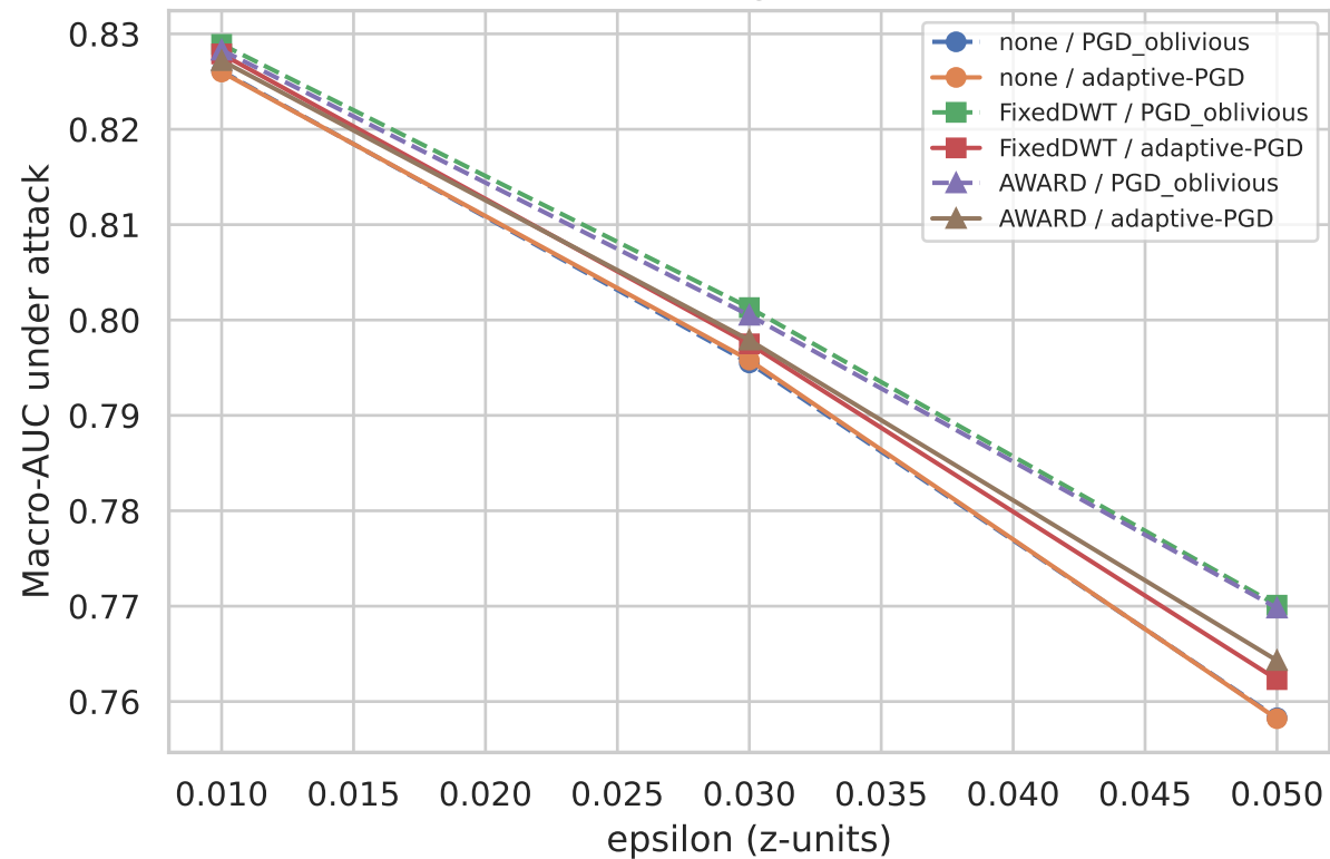
External robustness (Zheng subset, frozen defenses)
