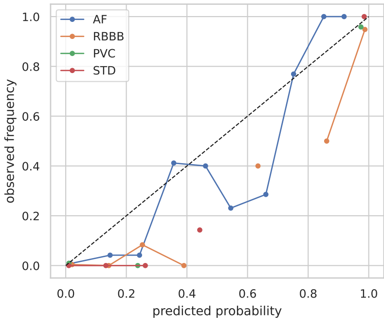
Reliability diagram (test; ECE=0.075)
