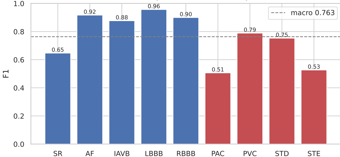
Per-class test F1 (final system; red = historically weak classes)
