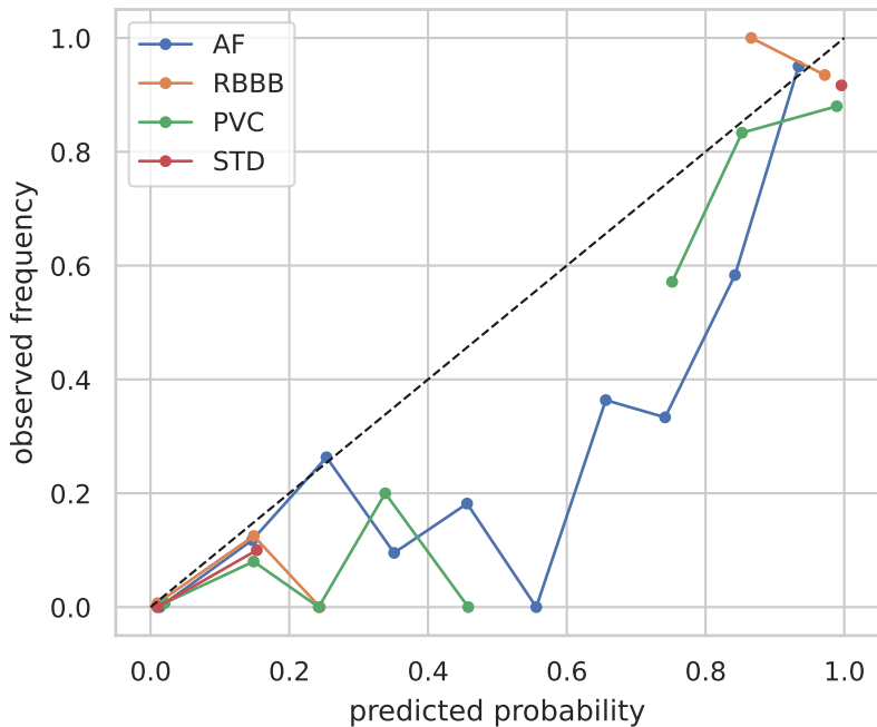
Reliability diagram (test; ECE=0.081)
