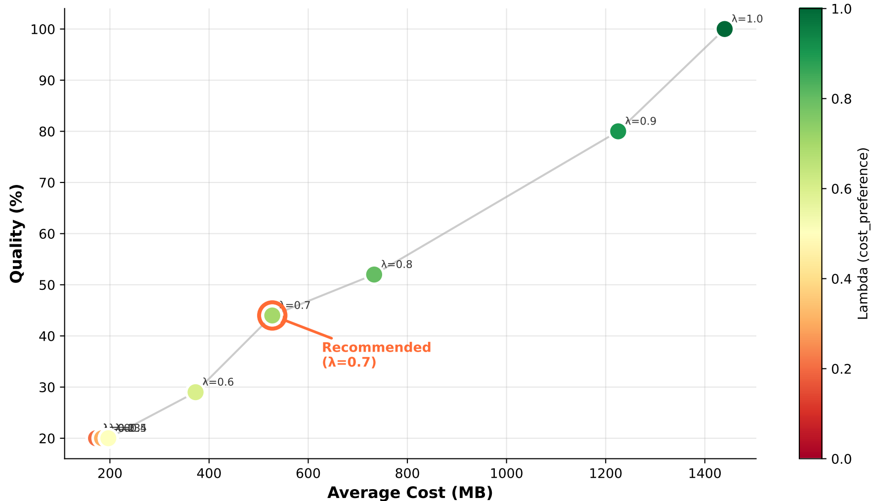
Quality-Cost Tradeoff (Each point is a different lambda value)
