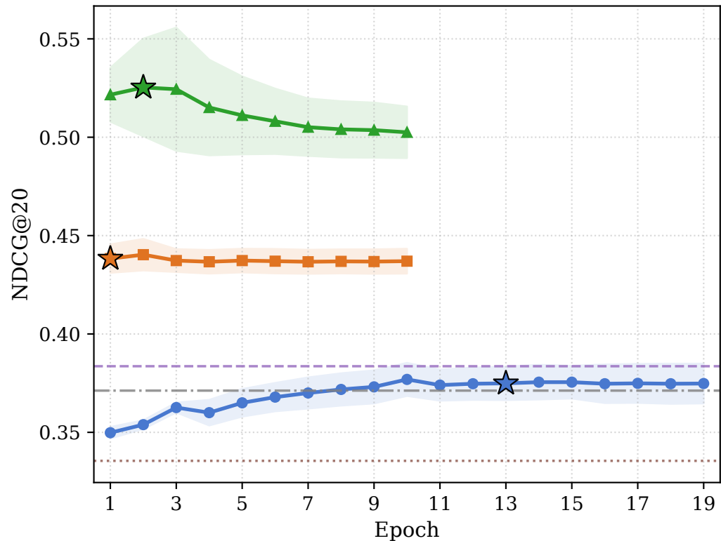
(b) NDCG@20 vs. Epoch
