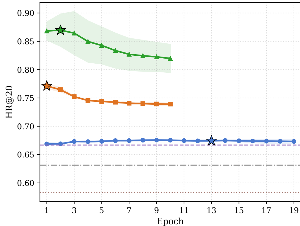
(a) HR@20 vs. Epoch
