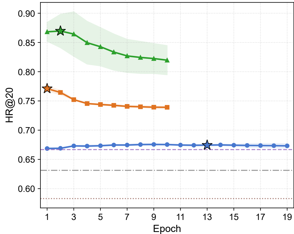
(a) HR@20 vs. Epoch
