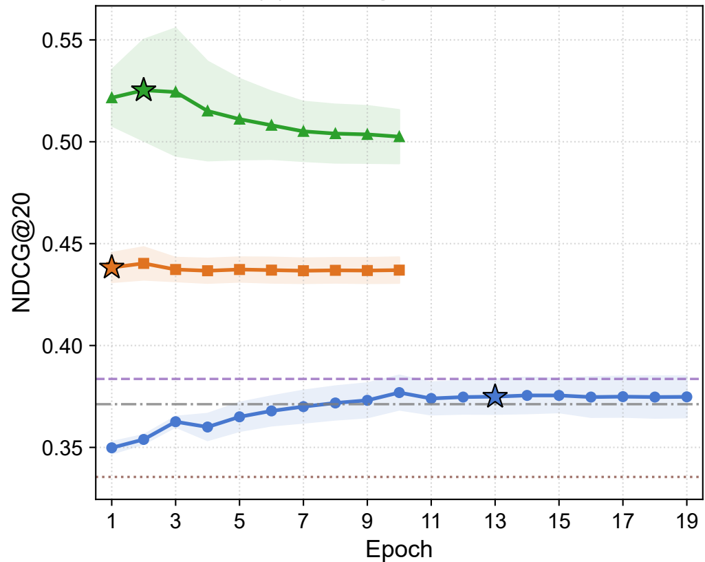
(b) NDCG@20 vs. Epoch
