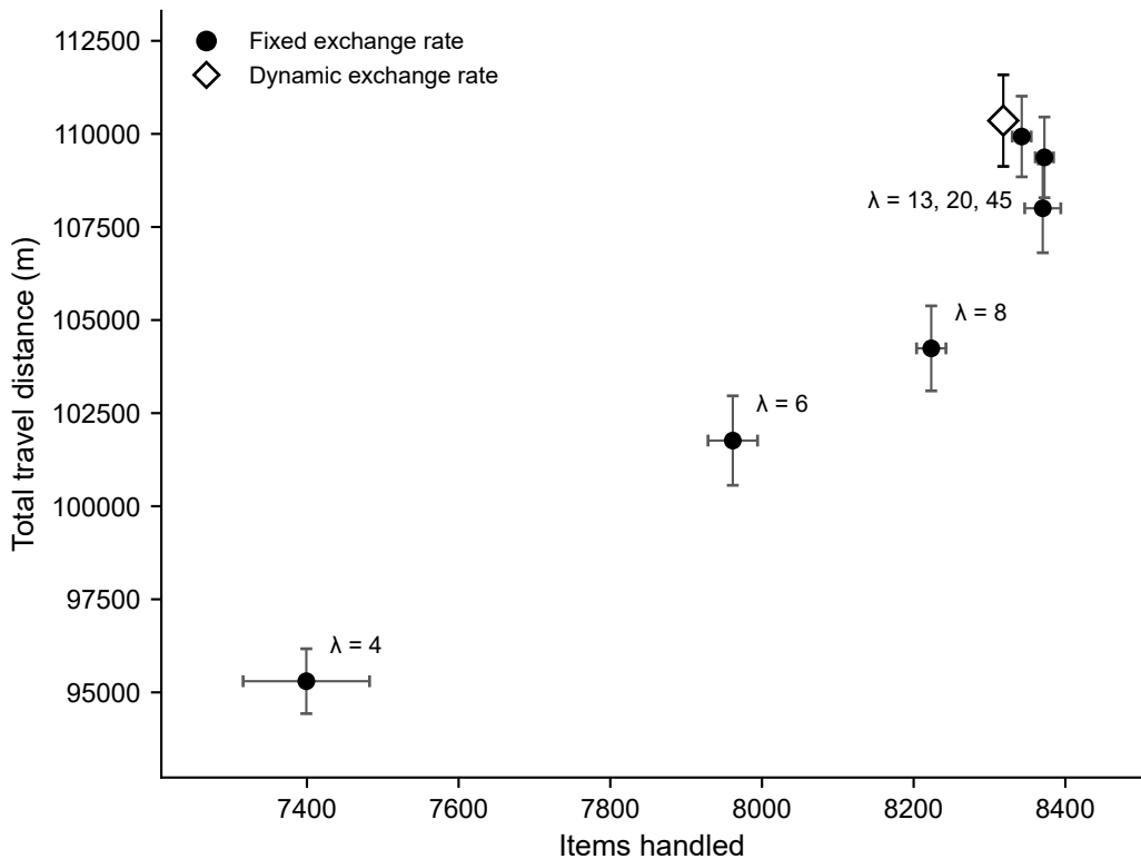
Fixed vs. Dynamic Exchange Rate: Distance and Throughput (45 Robots)
