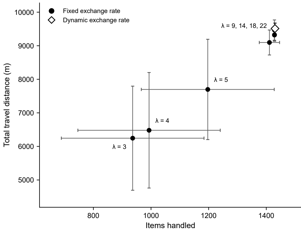
Fixed vs. Dynamic Exchange Rate: Distance and Throughput (10 Robots)
