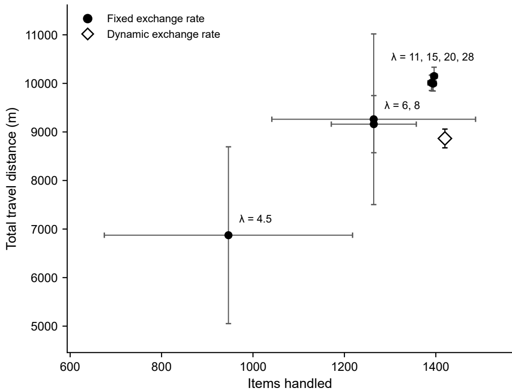
Fixed vs. Dynamic Exchange Rate: Distance and Throughput (6 Robots)
