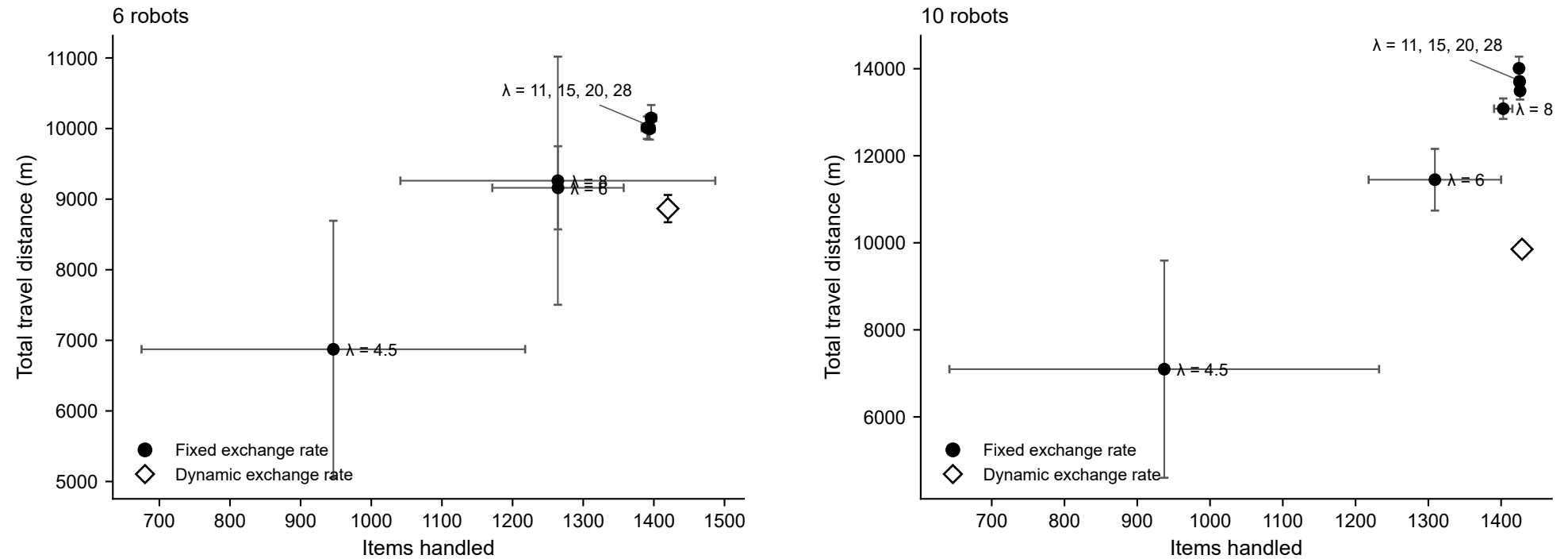
Figure 1 Total Travel Distance as a Function of Items Handled Under Fixed and Dynamic Exchange Rates
