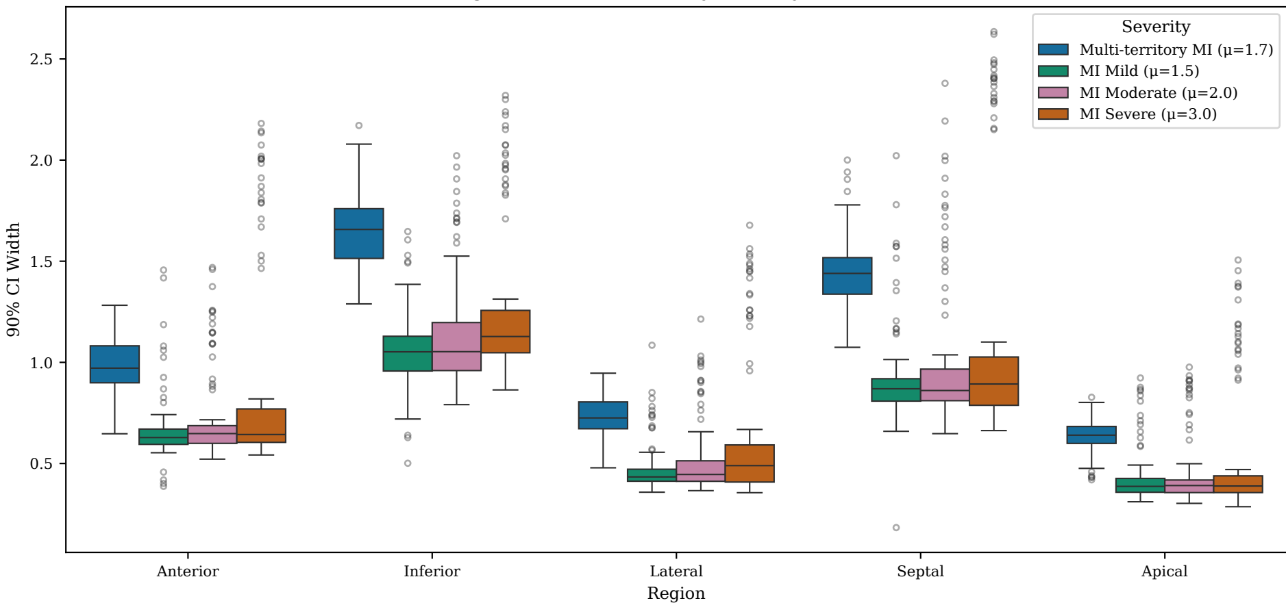
Regional 90% CI Width by Severity — MCMC
