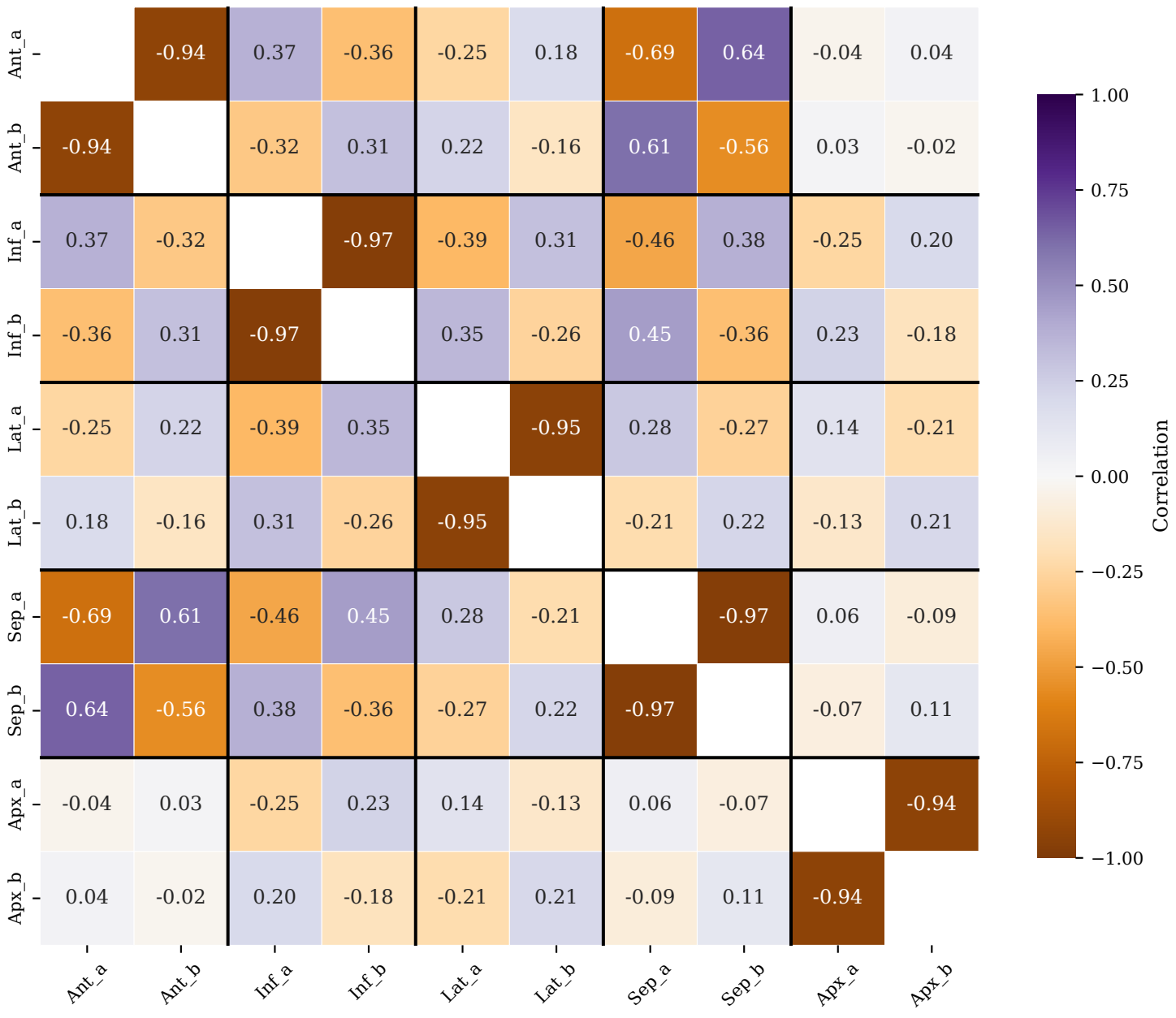
Full Parameter Correlation — Multi-territory MI ( \mu=1.7 )
