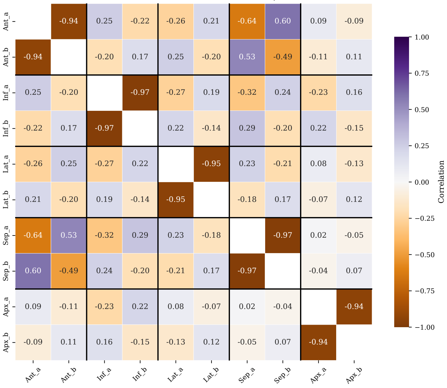
Full Parameter Correlation — MI Moderate ( \mu=2.0 )
