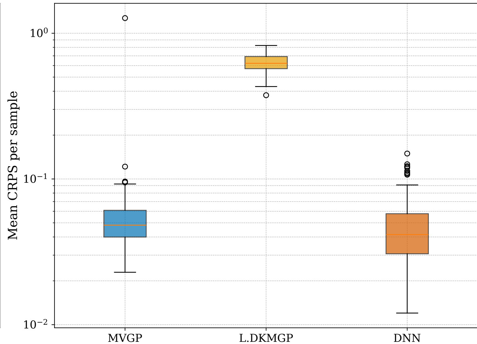
(b) Per-Sample CRPS Distribution (log)
