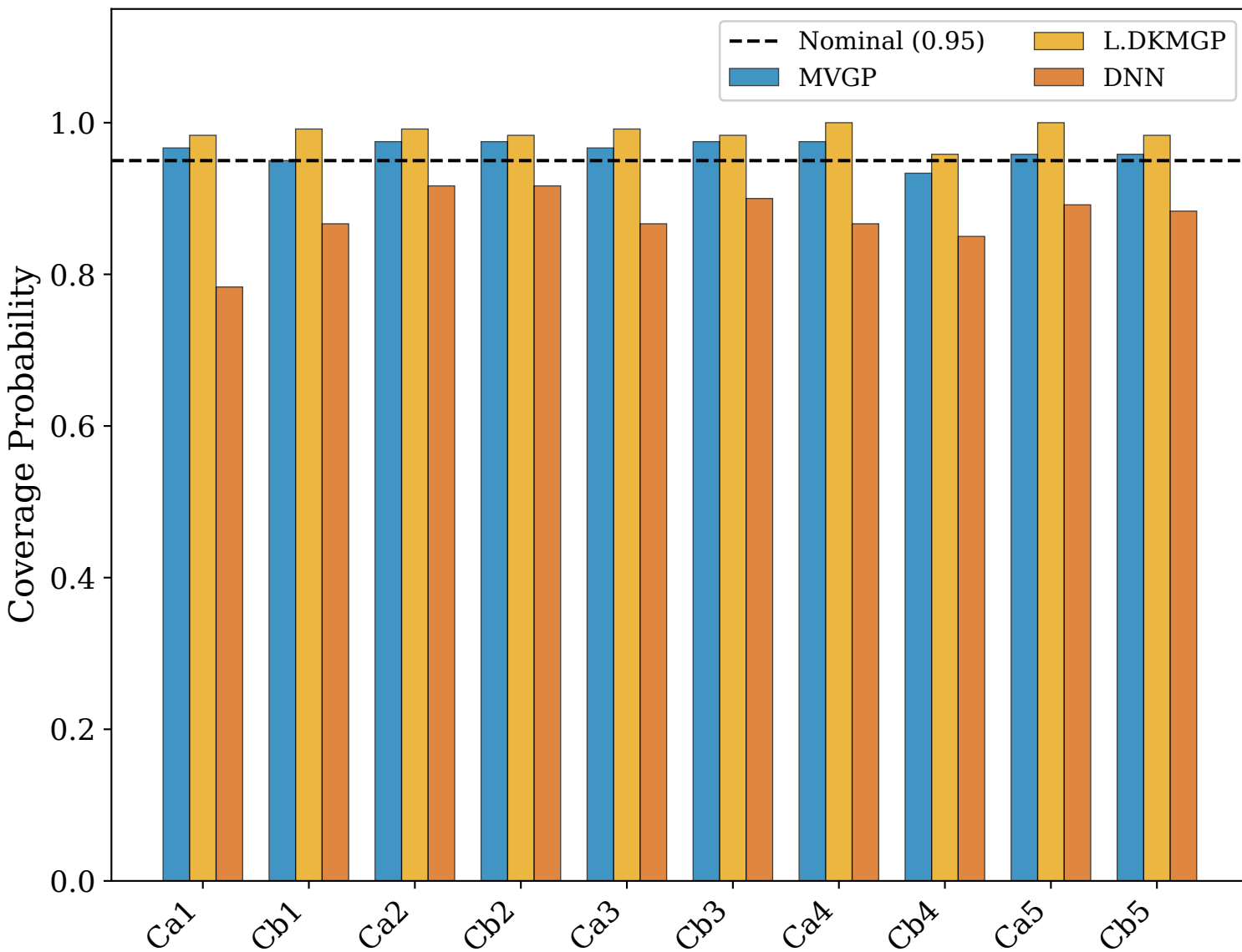
(a) 95% CI Coverage by Parameter
