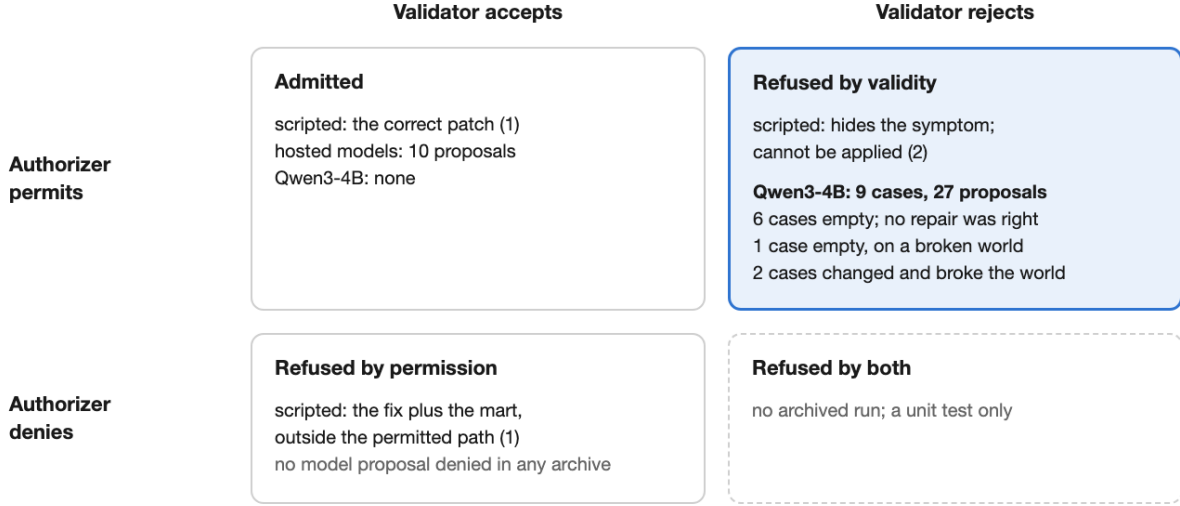
Figure 2: Every proposal that reached both checks: the scripted square, the hosted models' final packs and the local extension. Real proposals landed in two cells; no archived run was denied and rejected.
