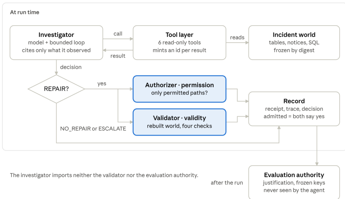
Figure 1: The system. Only a REPAIR meets the run-time checks; only the evaluation authority sees the key.
