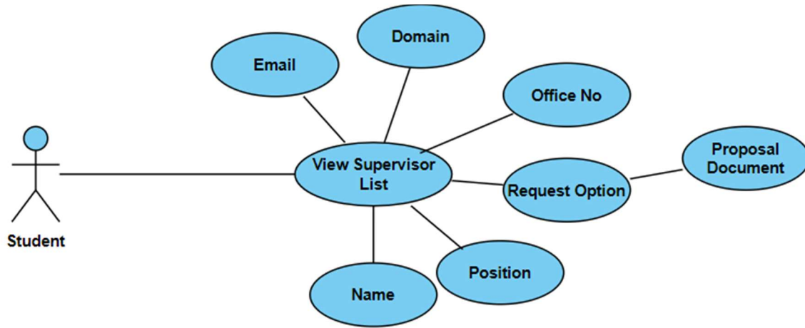
Figure 7 Use Case Diagram Request To Supervisor
