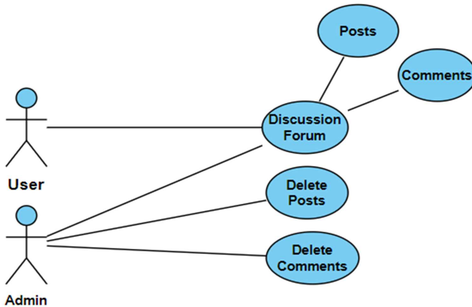
Figure 4 Use Case Diagram Discussion Forum
