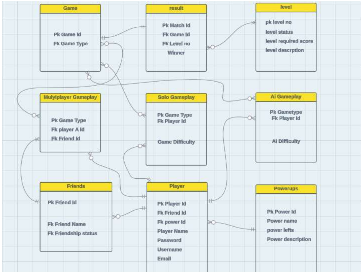
Figure 45 ERD
