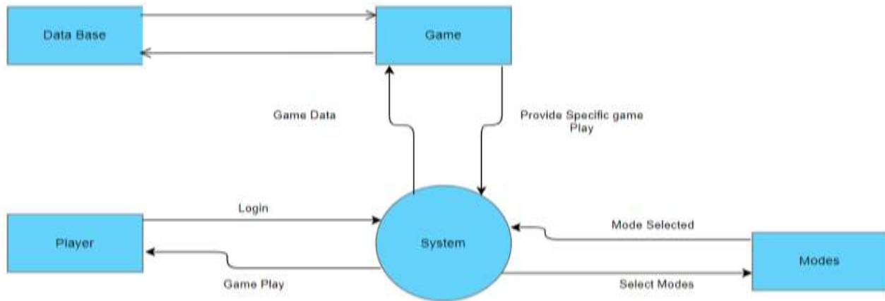
Figure 46 Level 0 DFD
