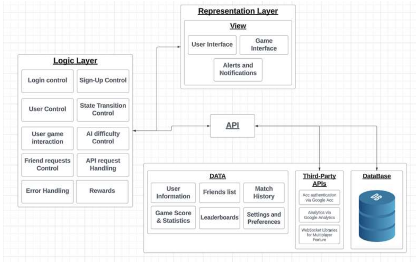
Figure 44 Architecture Diagram
