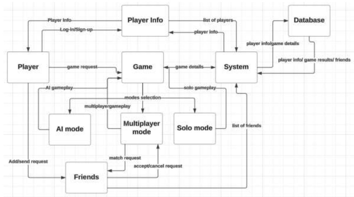
Figure 47 Level 1 DFD
