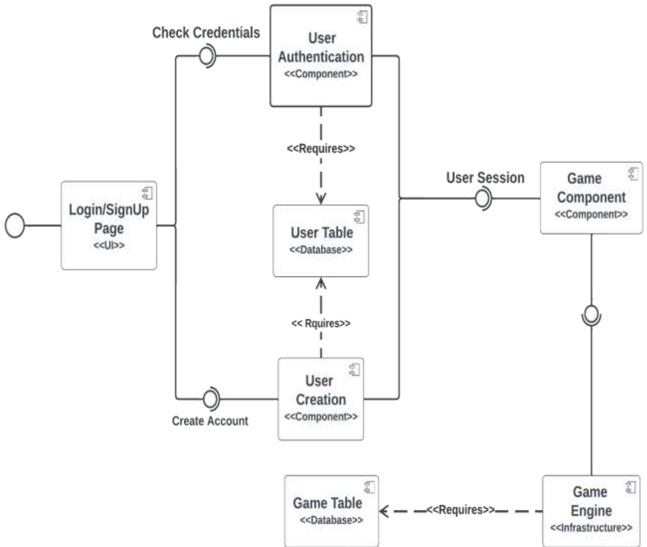
Figure 83 Component Diagram
