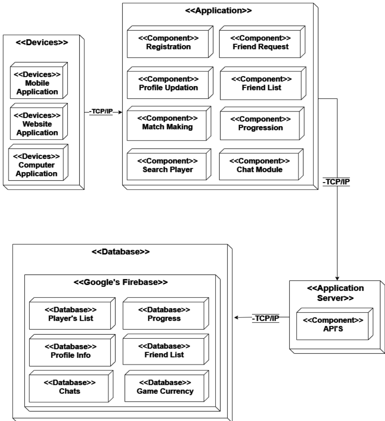
Figure 84 Deployment Diagram
