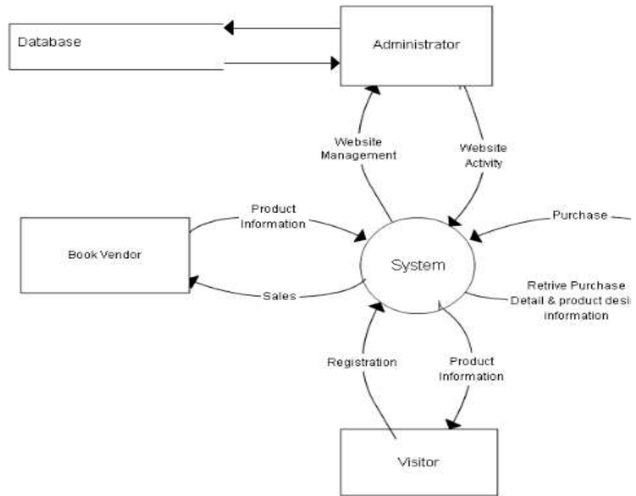
Figure 4 Level 0 DFD
