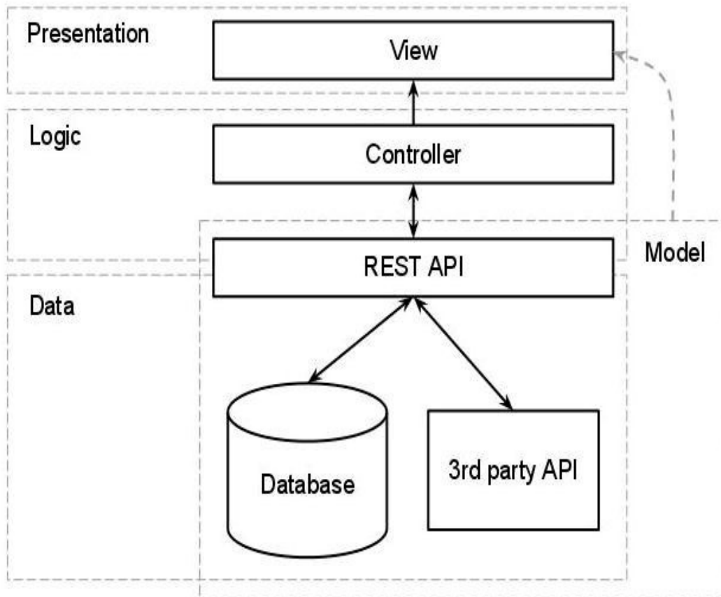
Figure 2 Architecture Diagram
