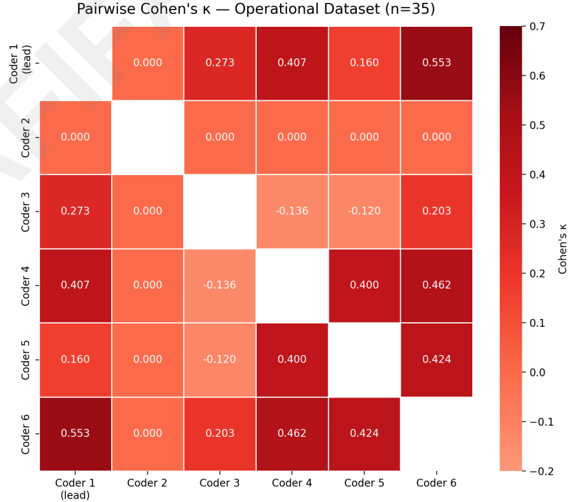
Figure 4.8: Pairwise Cohen's \kappa heatmap for six coders on the operational dataset.
