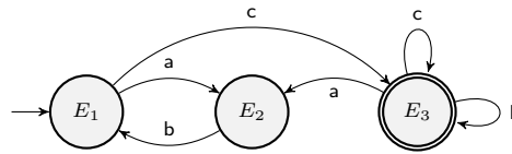
FIGURE 4 – Un automate ( A_2 )
