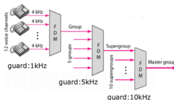
Figure 8: FDM hierarchy for Question 16
