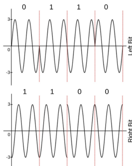
Figure 6: QPSK-modulated signal for Question 11
