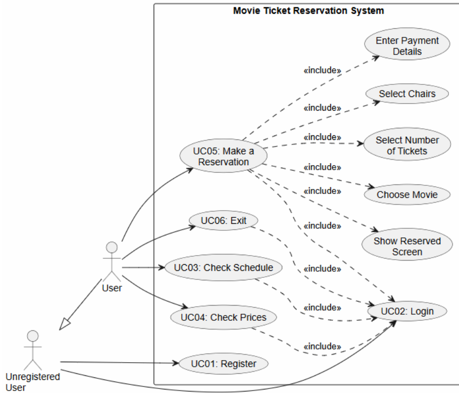
Figure 2 - Use Case Model
