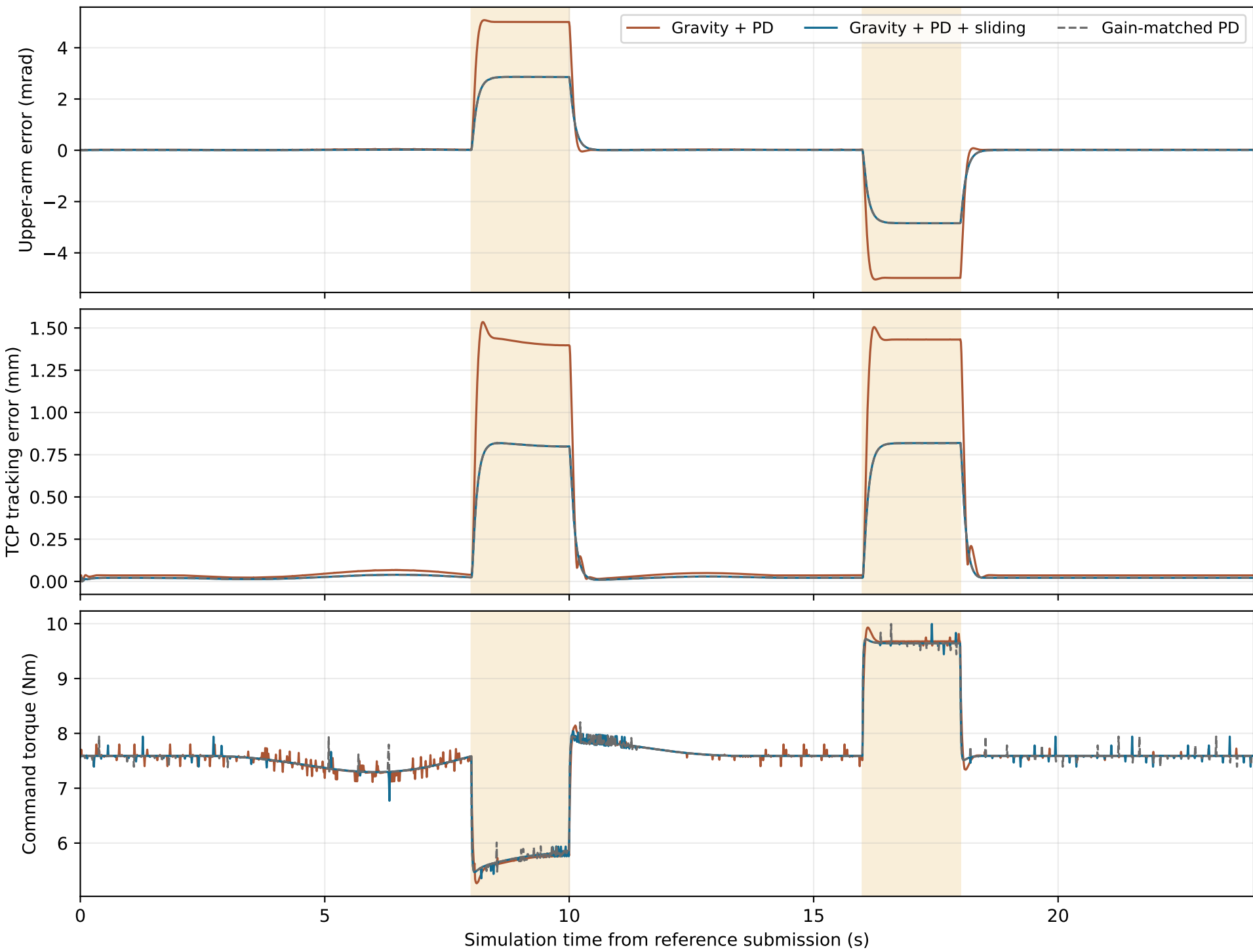
Gazebo effort control: external upper-arm torque +2 / -2 Nm Sliding feedback overlaps gain-matched PD in this boundary-layer experiment
