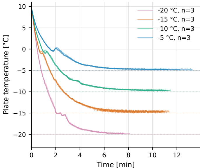
A Active dry-cooling telemetry
