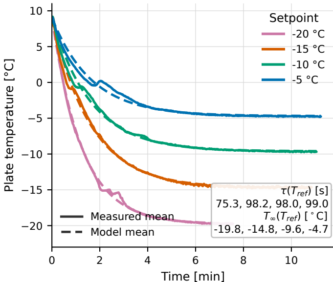
B Setpoint-dependent first-order fit
