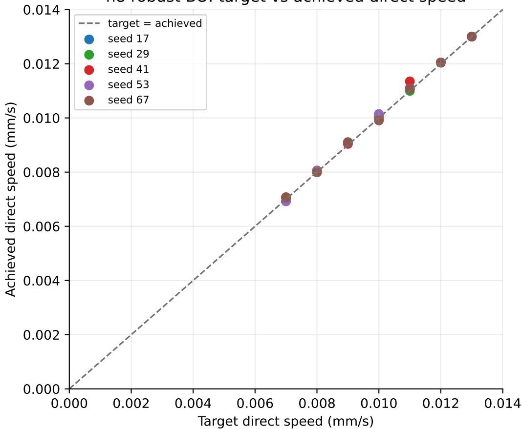
n8 robust BO: target vs achieved direct speed
