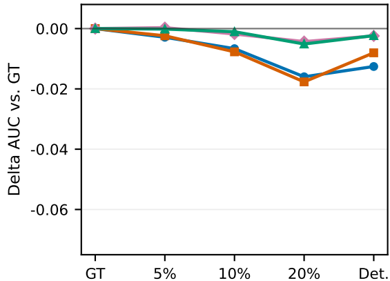
(b) Robustness loss
