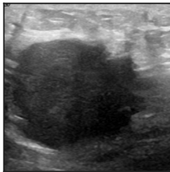
BUSI
