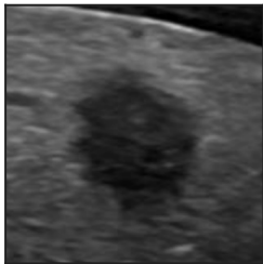
TN5000
