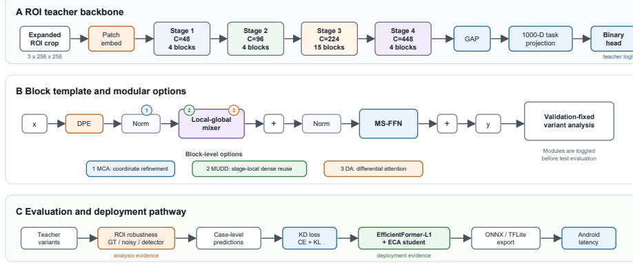
Figure 2: Overview of the ROI teacher-analysis and mobile-distillation workflow. (A) The TransXNet-family teacher processes expanded lesion ROIs through a four-stage local-global backbone and a binary task head. (B) Modular adaptations are analyzed inside representative blocks under validation-fixed model selection. (C) Teacher variants support ROI-robustness evaluation and distillation into an EfficientFormer-L1+ECA student for Android measurement.
