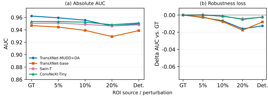
Figure 4: AUC robustness under GT boxes, synthetic perturbations, and detector-derived boxes. The left panel compares absolute AUC; the right panel shows degradation from each model’s GT-ROI AUC.
