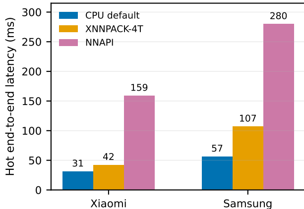
(b) Runtime backend sweep for ECA+KD
