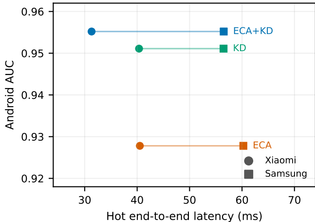
(a) Student accuracy-latency trade-off
