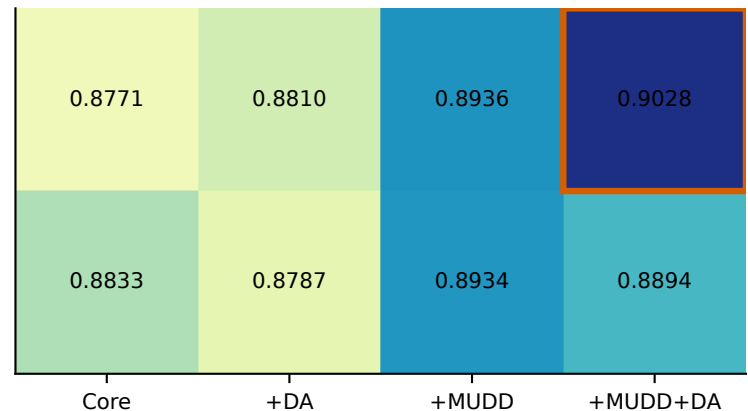
Ensemble balanced accuracy
