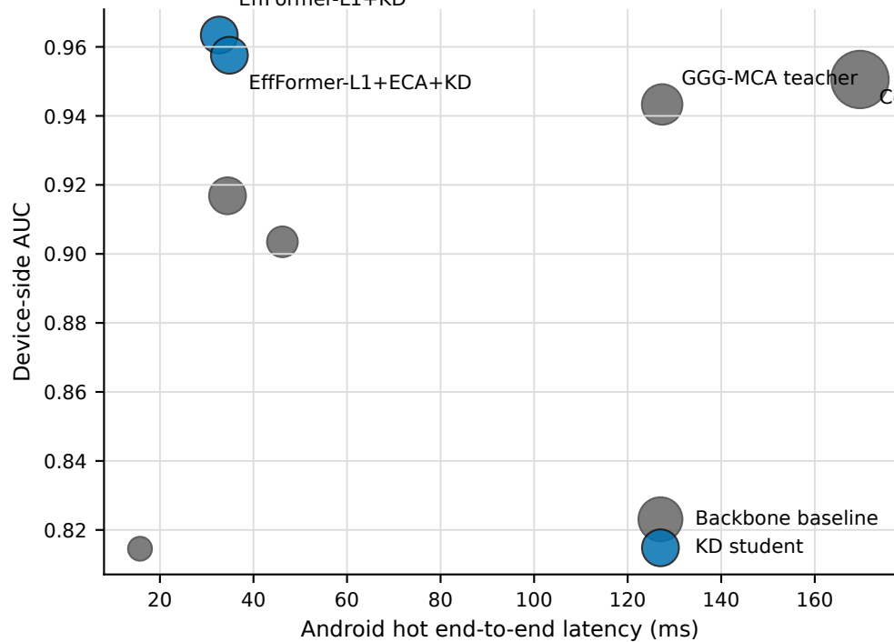
Android latency-performance trade-off
