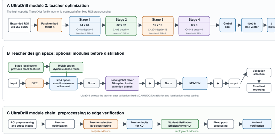
Figure 2: UltraDrill framework overview. (A) The teacher-optimization module uses a TransXNet-family four-stage local-global backbone for expanded lesion ROIs. (B) The teacher design space toggles coordinate-aware refinement, dynamic dense reuse, and differential attention before validation-fixed teacher selection. (C) The framework links fixed ROI preprocessing, teacher-family optimization, localization-stress testing, student distillation, ONNX export, and two-device Android verification.
