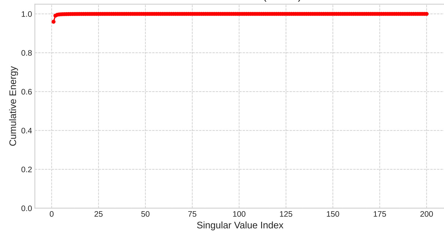
Cumulative Sum (Phase)
