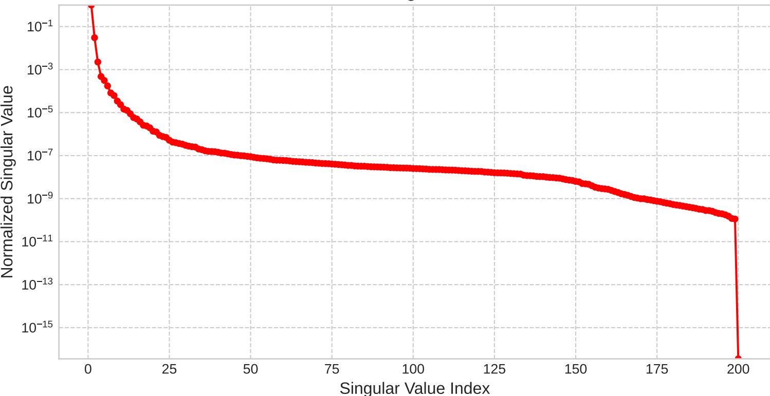
Phase Singular Values
