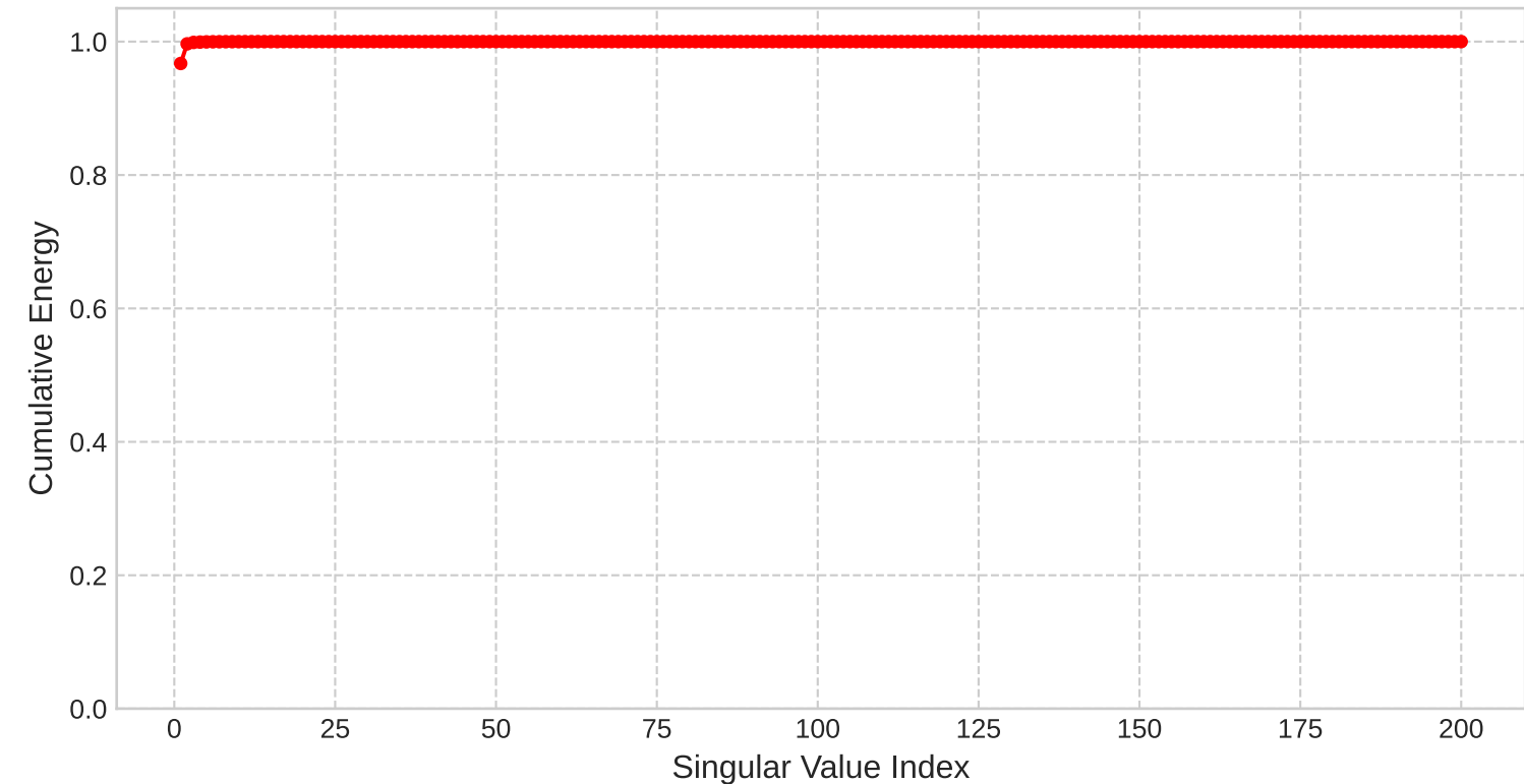
Cumulative Sum (Phase)
