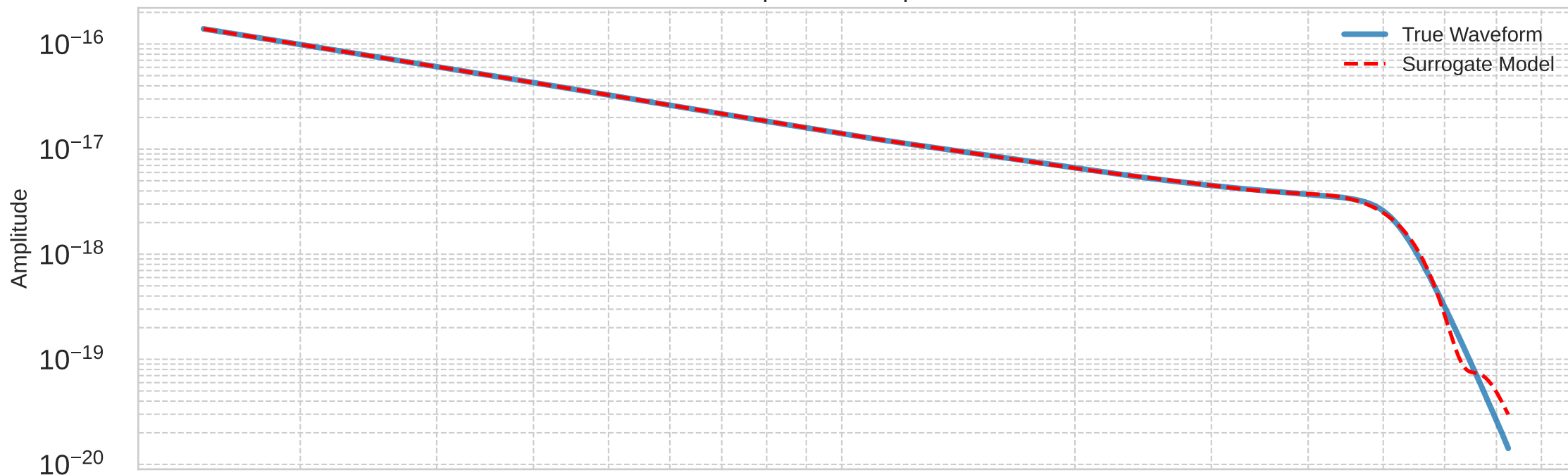
Amplitude Comparison
