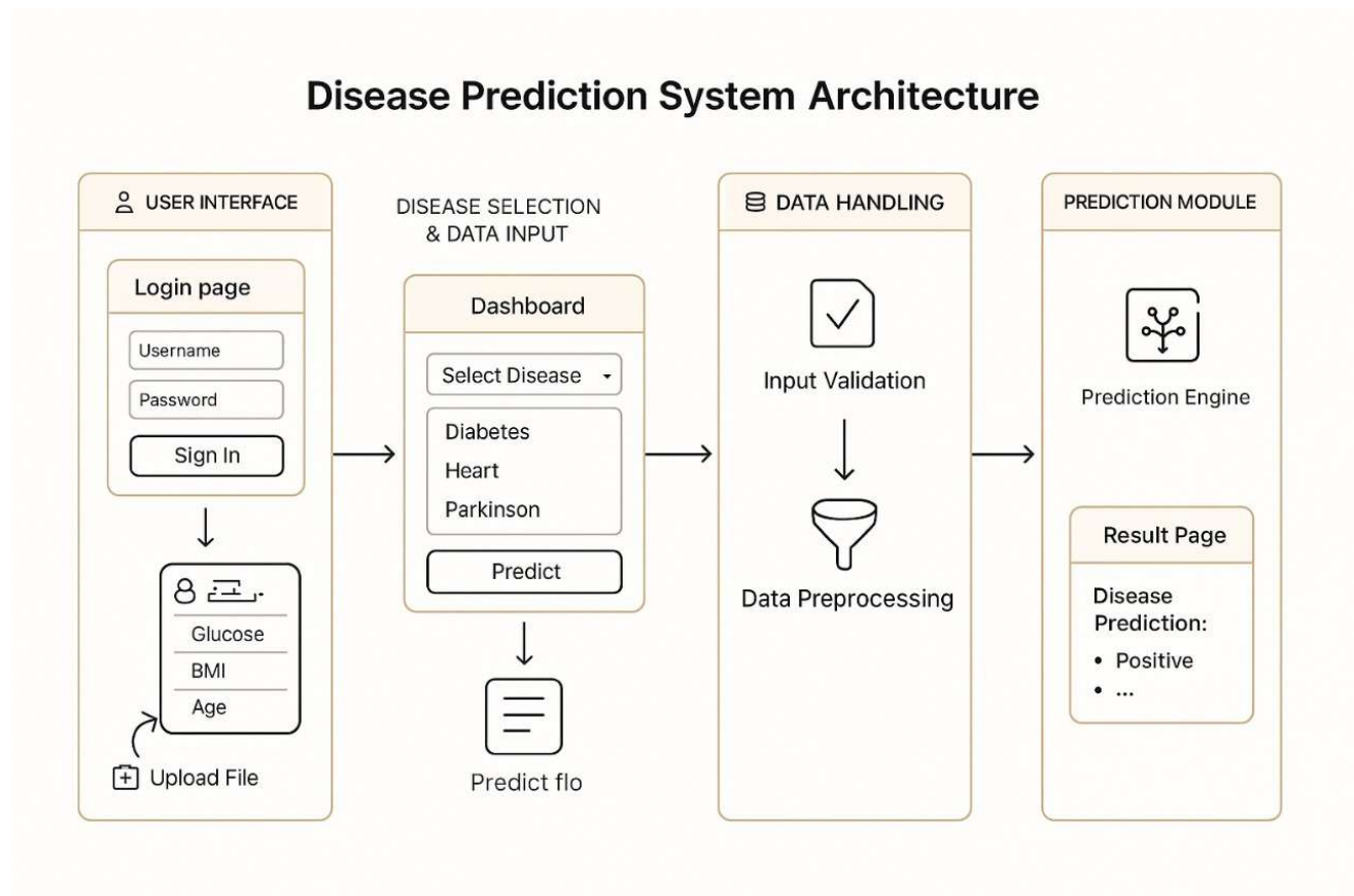
FIG 4.3 ARCHITECTURE DIAGRAM
