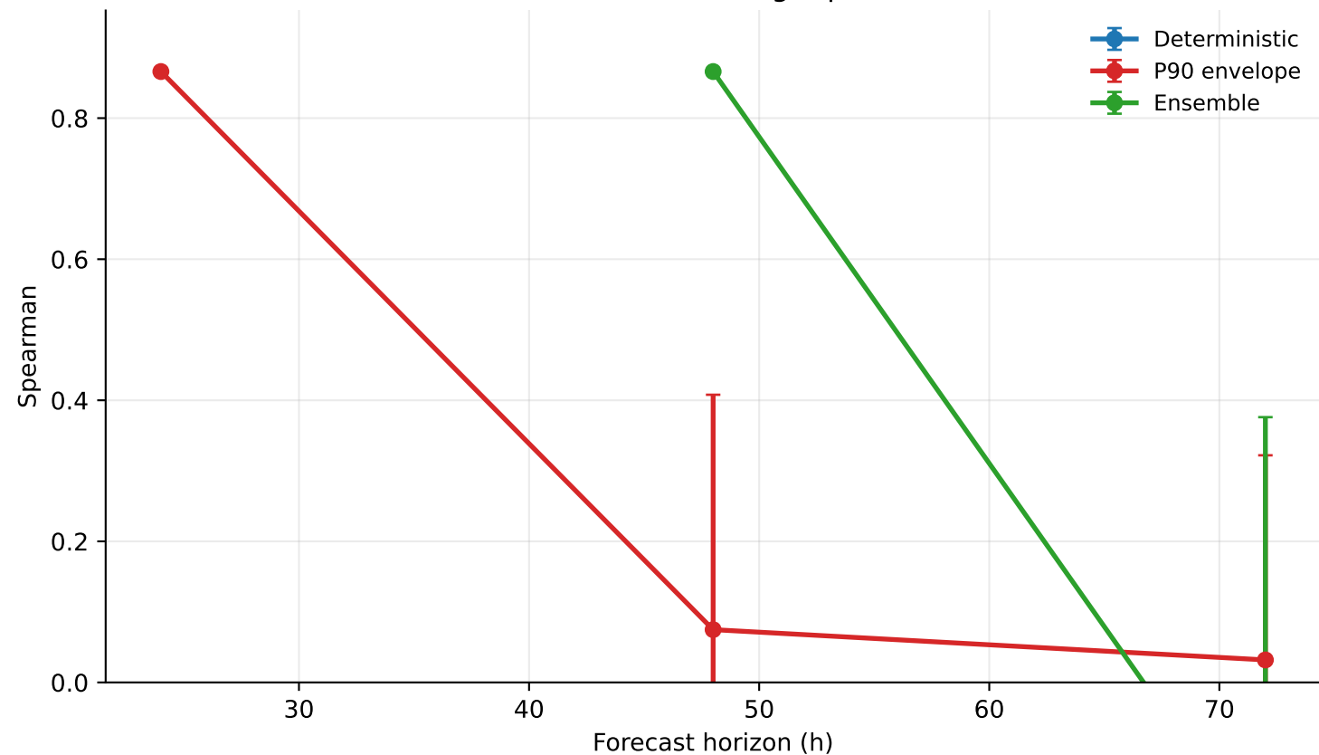
RQ3 real-data ranking: Spearman
