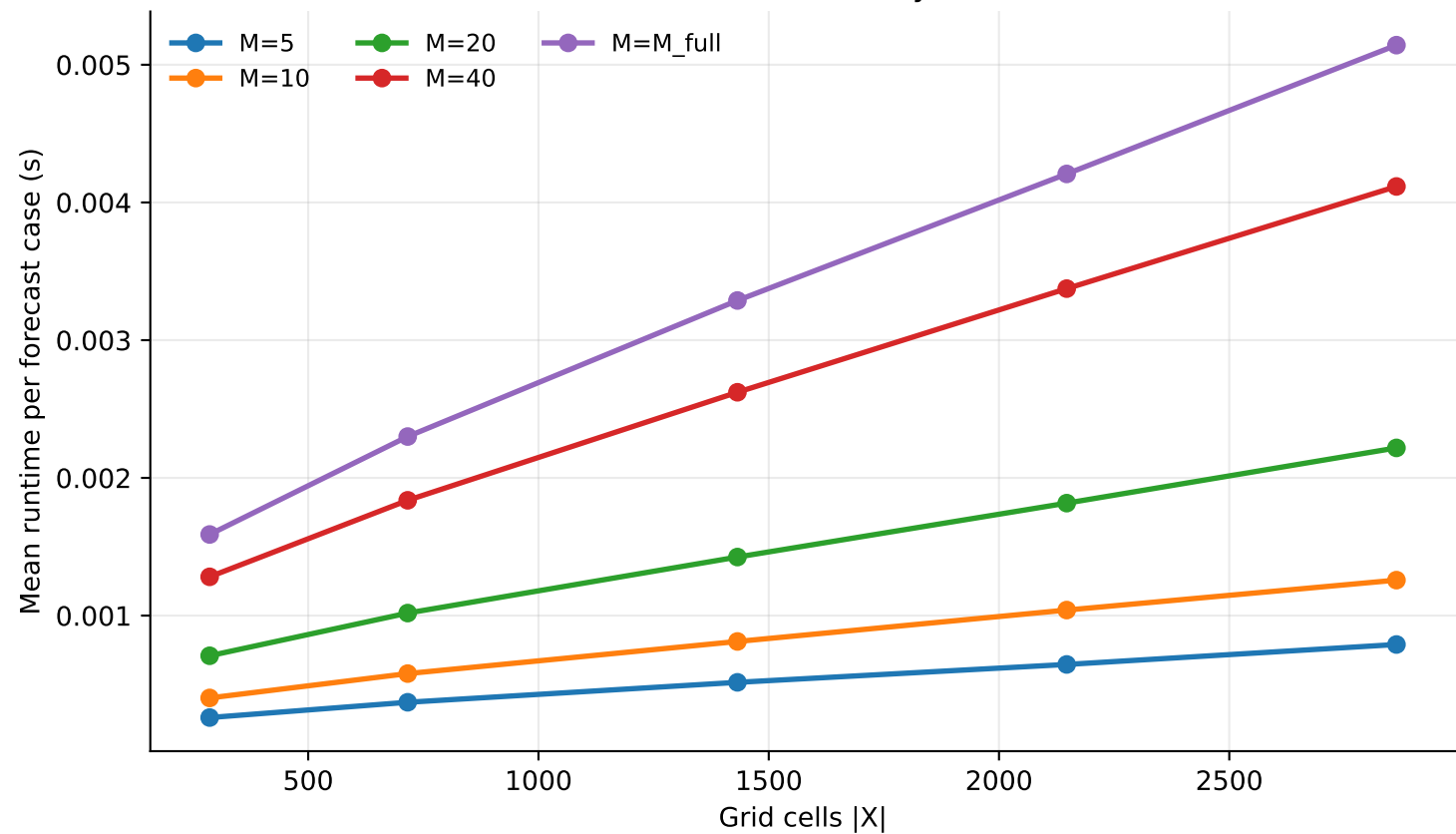
RQ4 real-data scalability runtime
