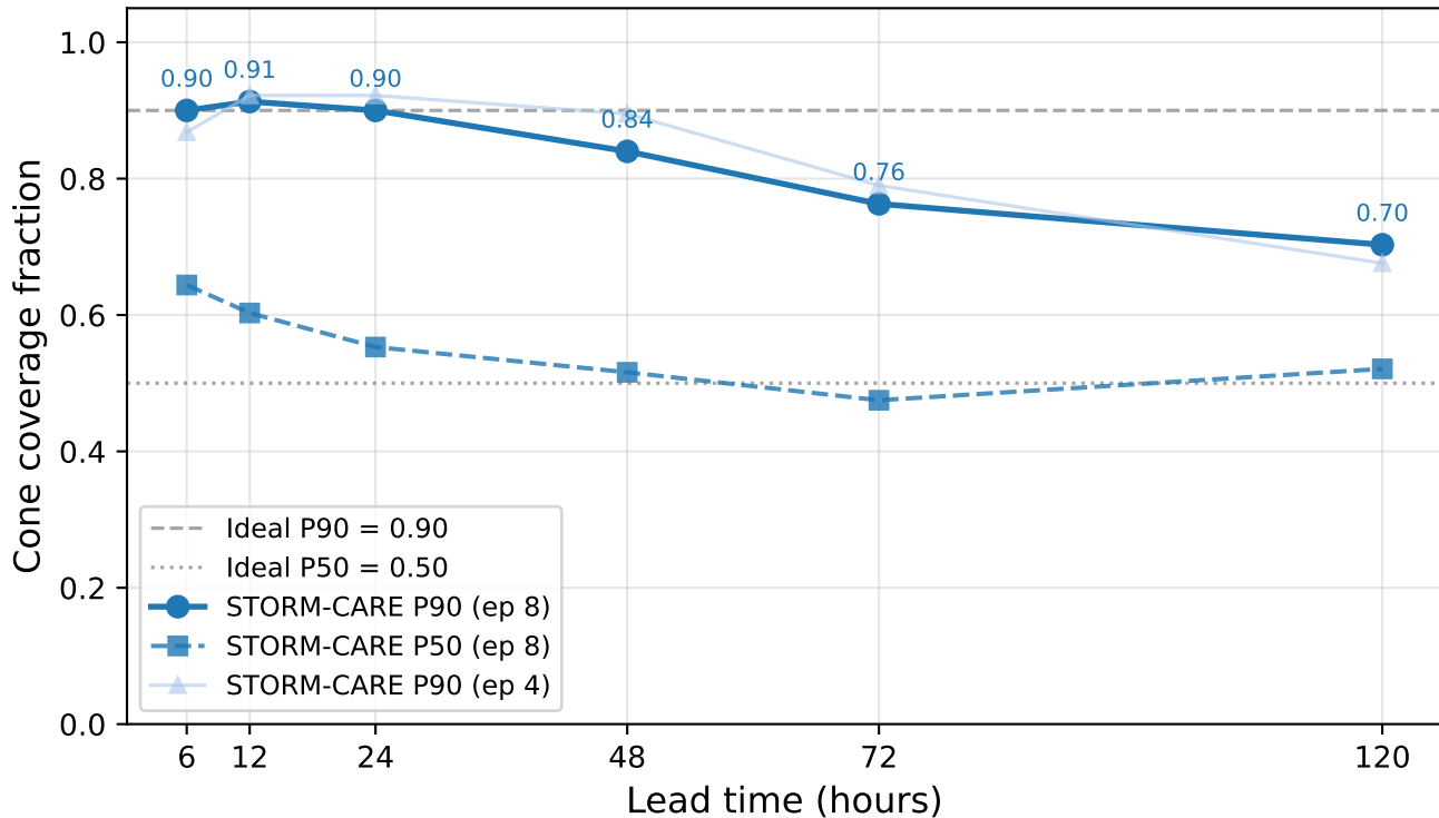
Forecast Cone Coverage vs Lead Time (STORM-CARE Foundation Model, validation set)
