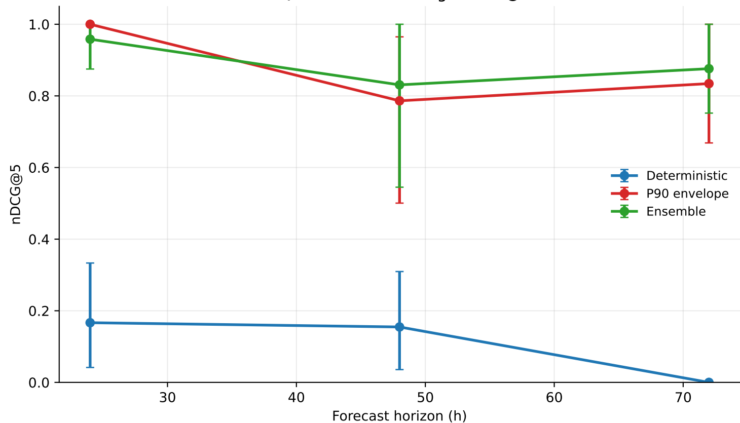
RQ3 real-data ranking: nDCG@5
